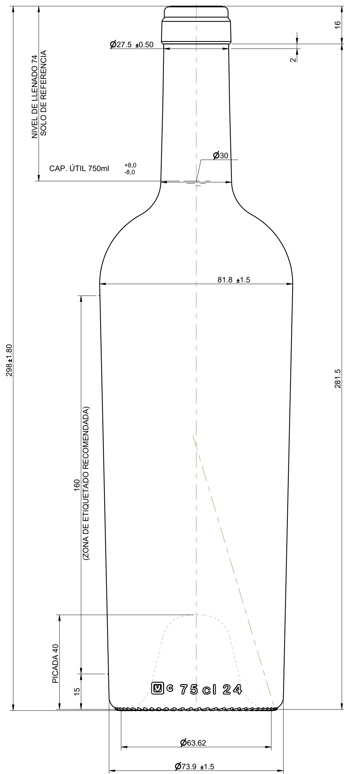
VISTA FRONTAL
