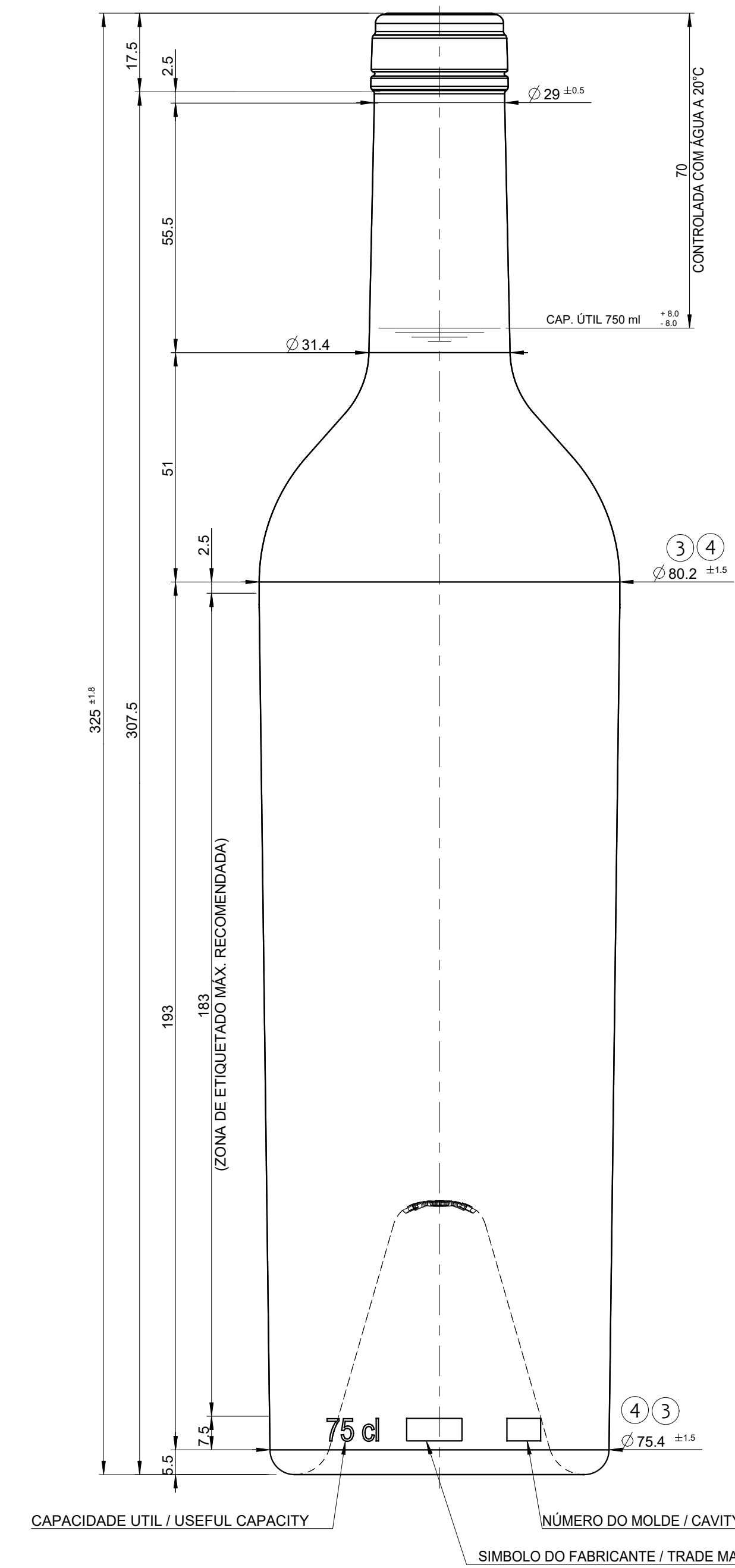
VISTA FRONTAL / FRONT VIEW
