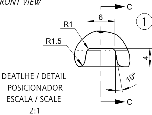
VISTA FRONTAL / FRONT VIEW
